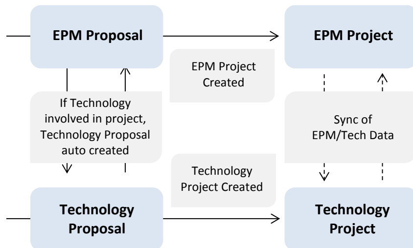
Figure 1. PPM design utilizes a Parent-Child relationship for proposals and projects
